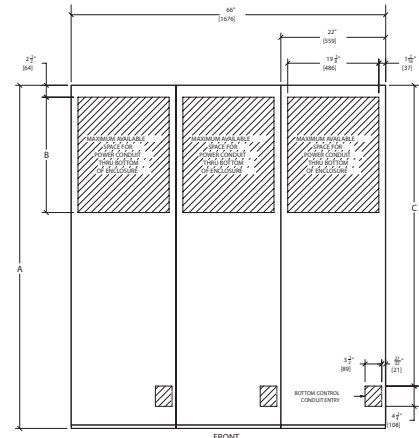
PLAN VIEW (3 SECTIONS)
